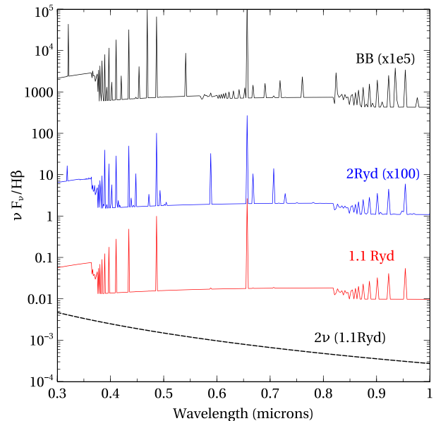
Figure 3. CLOUDY simulations of the emission spectrum of a mono-layer of He and H gas with He/H = 0.1 at 15 000 K and n_H = 10^4 \text{ cm}^{-3} illuminated by a 10^5 K BB and two mono-energetic ‘laser’ radiation fields at 1.1 and 2 Ryd, respectively (see the text). The H I two-photon radiation contribution is shown for the 1.1 Ryd case (dashed line). The incident continuum has been subtracted from the BB spectrum. The 2 Ryd and the BB spectra have been multiplied by 10^2 and 10^5 for clarity.
