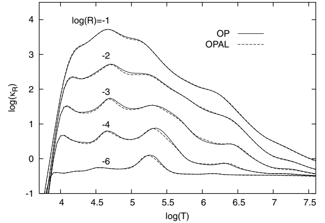
Figure 2. Rosseland-mean opacities from the OP and OPAL for the S92 mix.
