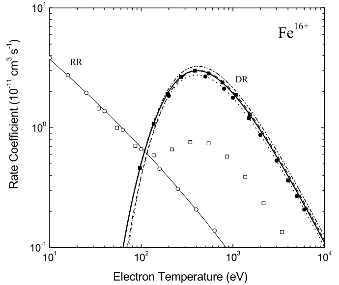
Fig. 3. Maxwellian-averaged DR and RR rate coefficients for recombination of \text{Fe}^{16+} to \text{Fe}^{15+} . Present results for DR (thick solid curve) and RR (thin solid curve) were obtained in the MCBP calculations with the code AUTOSTRUCTURE. Also shown are the MCDF results of Chen (1986, solid circles), which were used for the compiled data of Mazzotta et al. (1998, dotted curve), the FAC results of Gu (2003a, solid squares; 2003b, dash-dot-dotted curve), the results of Romanik (1988, dashed curve), the results of Jacobs et al. (1977, RR+DR, open squares), the RR results of Arnaud & Raymond (1992, open circles).
