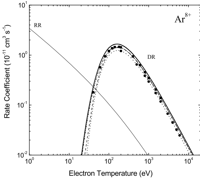
Fig. 2. Maxwellian-averaged DR and RR rate coefficients for recombination of \text{Ar}^{8+} to \text{Ar}^{7+} . Present results for DR (thick solid curve) and RR (thin solid curve) were obtained in the MCBP calculations with the code AUTOSTRUCTURE. Also shown are the MCDF results of Chen (1986, solid circles), which were used for the compiled data of Mazzotta et al. (1998, dotted curve), the FAC results of Gu (2003b, dash-dot-dotted curve), the results of Romanik (1988, dashed curve), and the results of Fournier et al. (1997, solid squares) using the fully relativistic, parametric potential atomic structure code RELAC.
