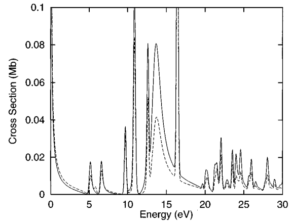
FIG. 3. Seven LS term R -matrix calculation for the \text{Sc}^{3+} recombination cross section including the 3p^5 3d^2 and 3p^5 3dn ( n > 3 ) resonances. Solid curve is in the length gauge, dashed curve is in the velocity gauge.
