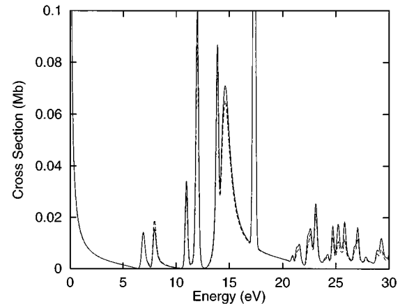
FIG. 4. Correlated seven LS term R -matrix calculation for the \text{Sc}^{3+} recombination cross section including the 3p^5 3d^2 and 3p^5 3dn ( n > 3 ) resonances. Solid curve is in the length gauge, dashed curve is in the velocity gauge.
