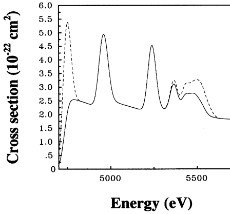
FIG. 1. Electron-impact excitation cross section for the 1s^2(^1S_0) \rightarrow 1s2p(^3P_1) (Y) transition in \text{Ti}^{20+} . Results are from a 17-level R -matrix calculation, convoluted with a 50 eV FWHM Gaussian. Solid line: radiative damping potential included; dotted line: no radiative damping.
