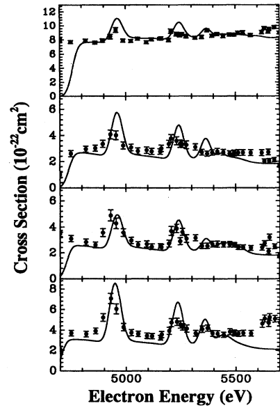
FIG. 4. R -matrix results for the electron-impact excitation cross section in Ti^{20+} : (a) 1s^2(^1S_0) \rightarrow 1s2p(^3S_1) ( Z ) transition; (b) 1s^2(^1S_0) \rightarrow 1s2p(^3P_1) ( Y ) transition; (c) 1s^2(^1S_0) \rightarrow 1s2p(^3P_2) ( X ) transition; (d) 1s^2(^1S_0) \rightarrow 1s2p(^1P_1) ( W ) transition. Experimental results from the EBIT experiment [13] are shown as solid circles.
