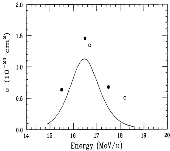
FIG. 5. RTE cross sections for \text{Kr}^{34+} + \text{H}_2 : ●, present data; ○, Ref. [13]. The solid curve is the calculated RTE cross section. The statistical errors are about the size of the symbols; the overall systematic uncertainty is estimated to be less than about 30%.
