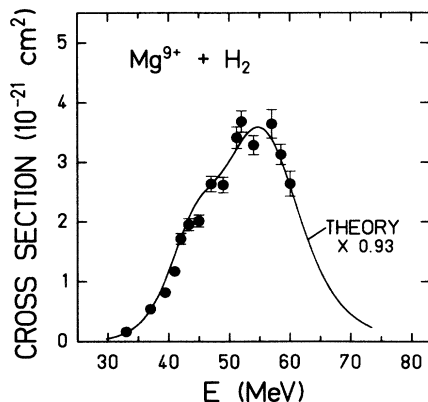
FIG. 3. Experimental cross sections (solid points) for K -shell x rays coincident with electron capture for Mg^{9+} + H_2 . Relative uncertainties are indicated. The present theoretical IC RTE calculations for this collision system (solid curve) have been multiplied by 0.93 to facilitate comparison with the data.
