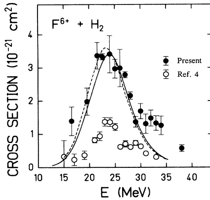
FIG. 2. Cross sections for K -shell x rays coincident with electron capture for F^{6+} + H_2 . The present measurements are indicated with solid points; the previous results from Ref. [4] are shown with open circles. Relative uncertainties are indicated. The present theoretical IC RTE calculations are shown by the solid curve, and the IC calculations of Bhalla and Karim (Ref. [5]) are shown with the dashed curve.
