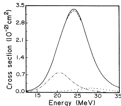
FIG. 1. Theoretical RTEX cross sections for F^{6+} + H_2 . —, intermediate coupling for KLn + KMn ( n \geq L ); - - -, LS coupling for KLn + KMn ( n \geq L ); - · - · -, intermediate coupling for KLL ; · · · ·, intermediate coupling for KMn ; all this work. The projectile energy is in the laboratory system.
